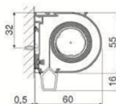
Pose face
